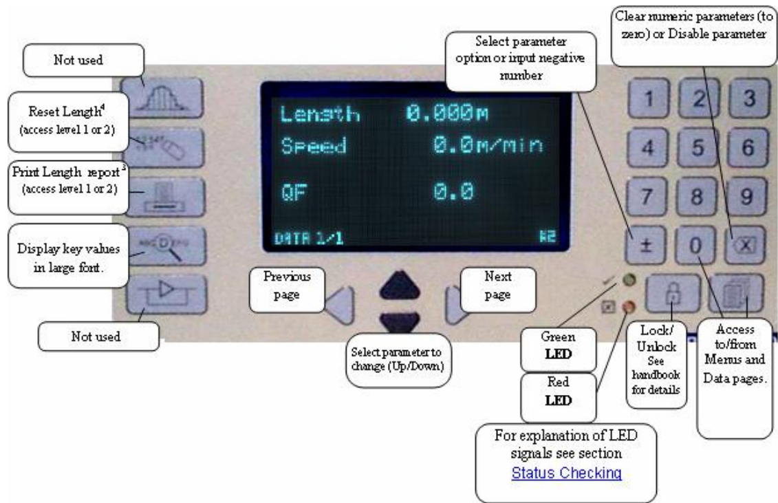
Figure 2 DP 1000 front panel
