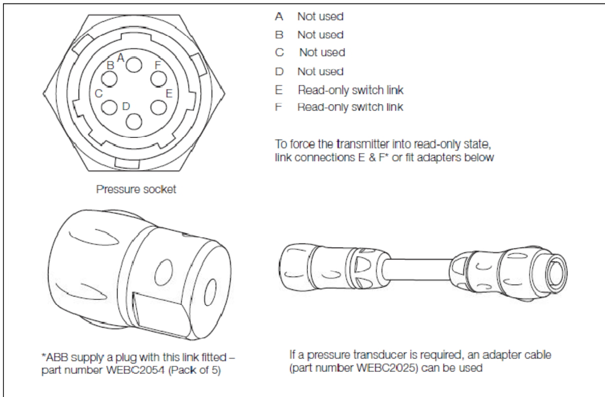
Figure 3 Transmitter “Metrological Read Only” Link
